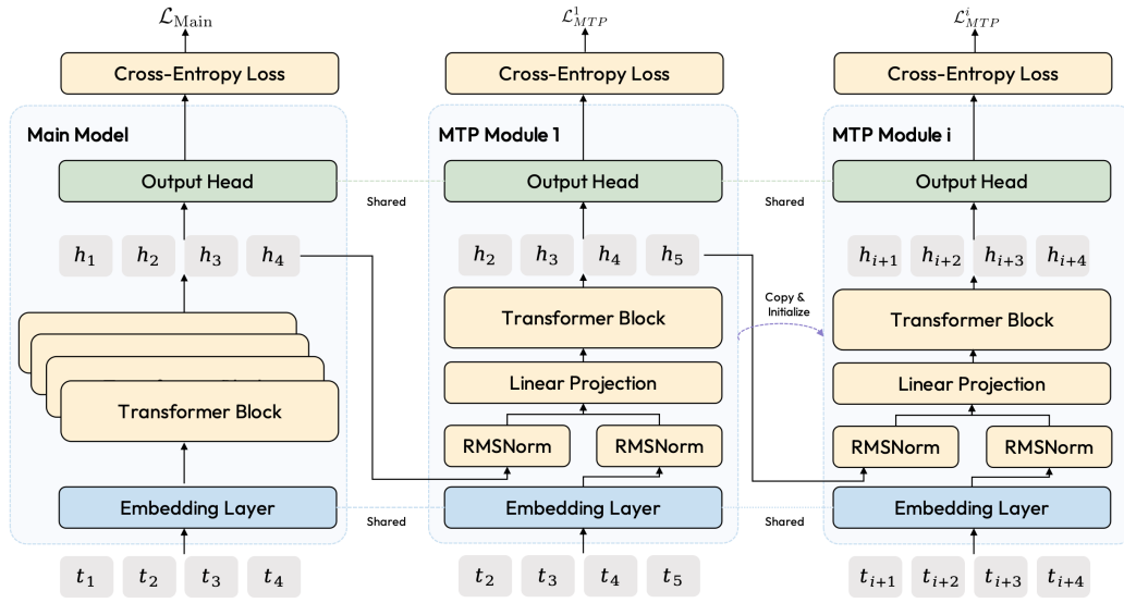
Figure 2 | Multi-Token Prediction (MTP) module architecture used in M2.
