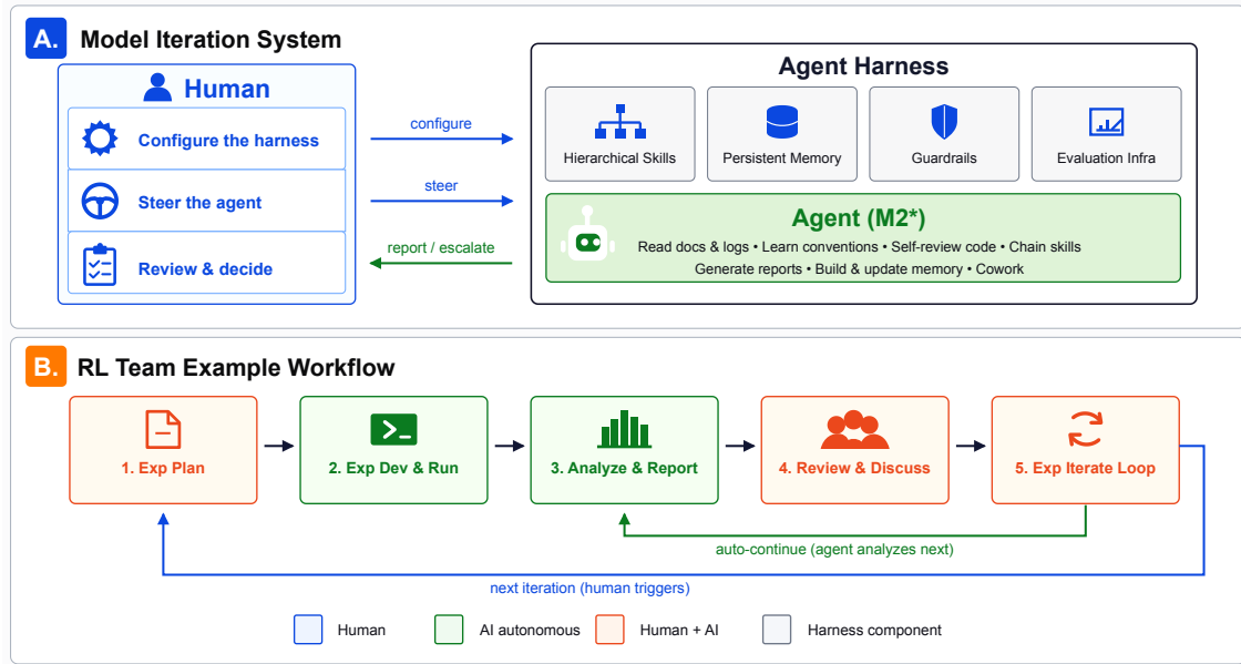
Figure 8 | (A) The Model Iteration System used to drive M2.7’s autonomous execution. (B) The dual-loop workflow used by our RL team.
